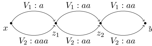
Figure 4: Example 14: An arbitrary database D whose view satisfies T(x, y) . Each arrow of the form V_i : w from a node u to a node v should be understood as a path from u to v whose label is w which witnesses (u, v) \in V_i(D) .
