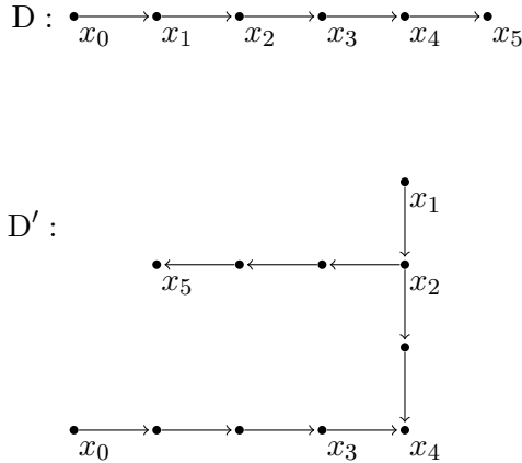
Figure 1: Illustration for Example 2: D and D' are such that \mathbf{V}(D) \subseteq \mathbf{V}(D') , but (x_0, x_5) \in Q(D) , whereas (x_0, x_5) \notin Q(D') . Hence the function induced by Q using \mathbf{V} is not monotone.
