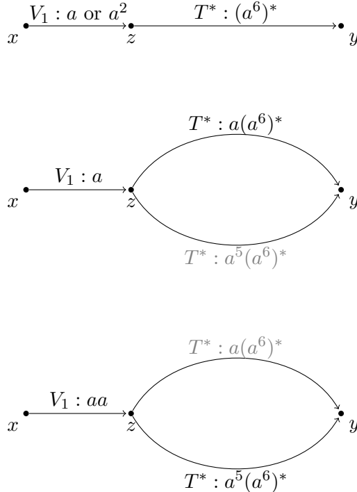
Figure 5: The three cases of Example 14. The parts that are not used for Q are shaded out.
