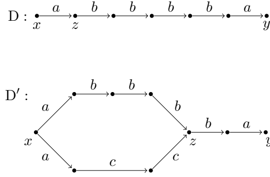
Figure 3: Databases D and D' for Example 13.
