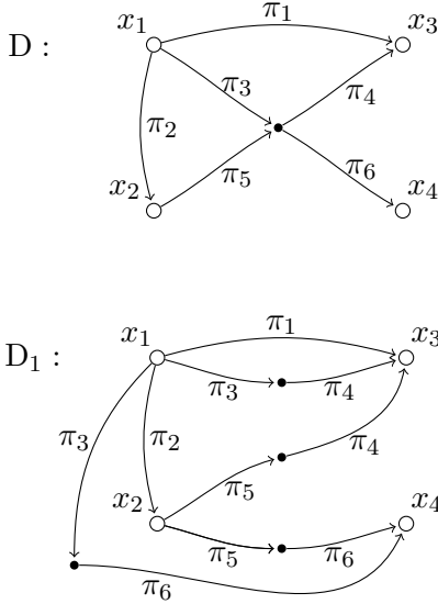
Figure 2: Illustration of the transformation from D to D_1 in Lemma 6. Nodes are colored white or black depending on whether they appear in \mathbf{V}(D) or not.
